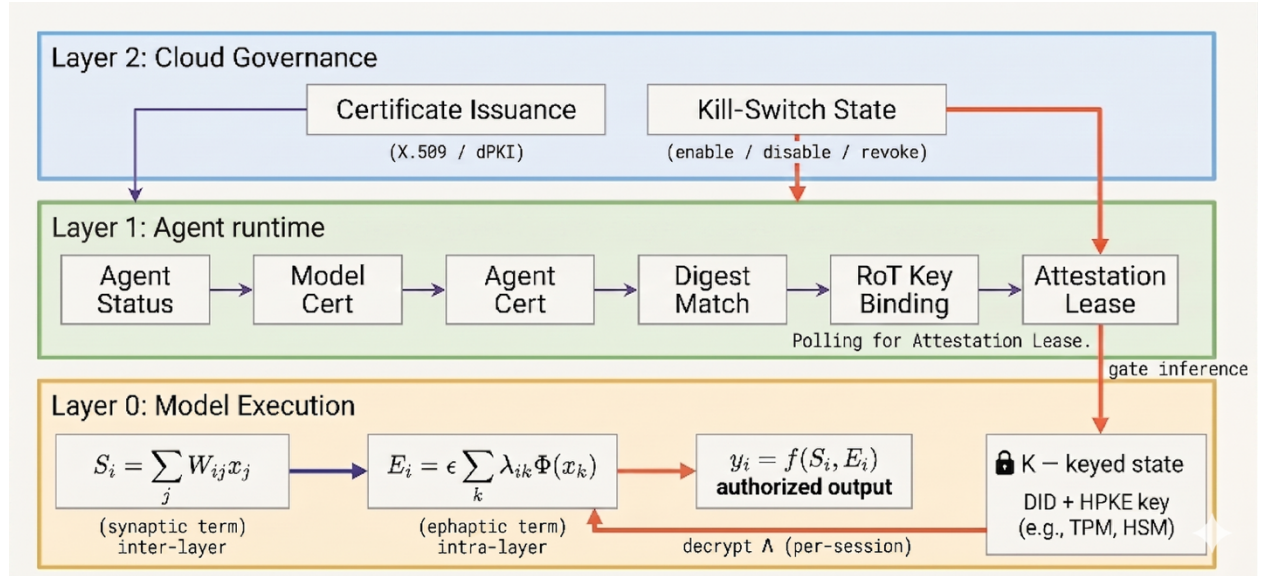
Figure 2: End-to-End Execution Pipeline
