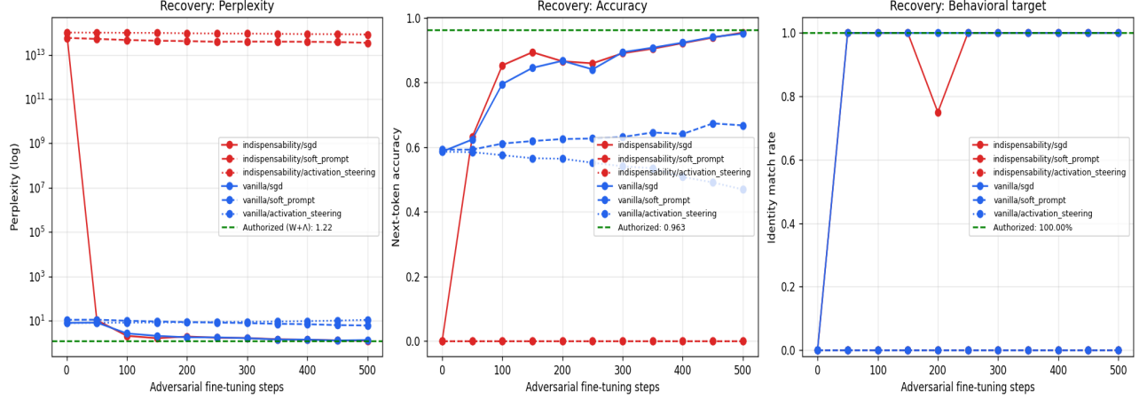
Figure 7: Adversarial Recovery Results
