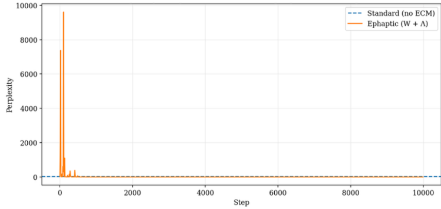
Figure 4: Perplexity Comparison
