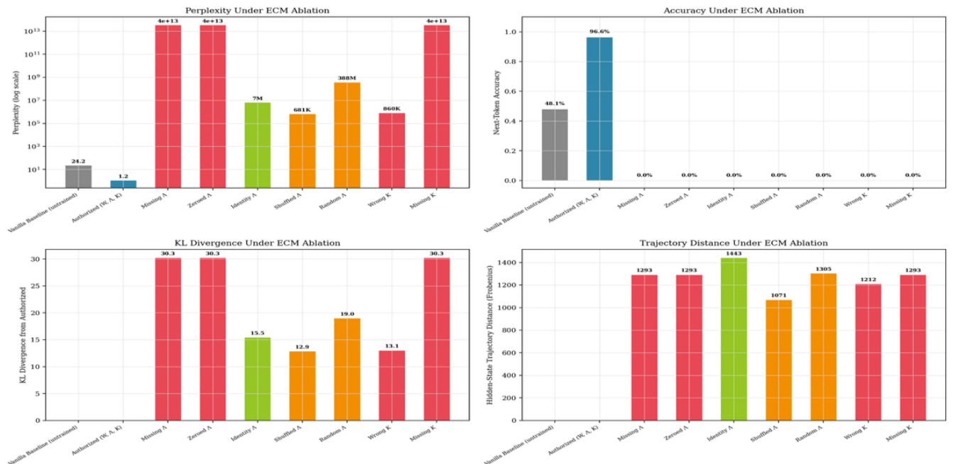
Figure 6: ECM Ablation Results
